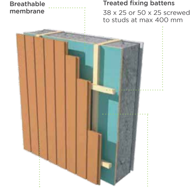
Vertical boards Fastened at every intermediary support
